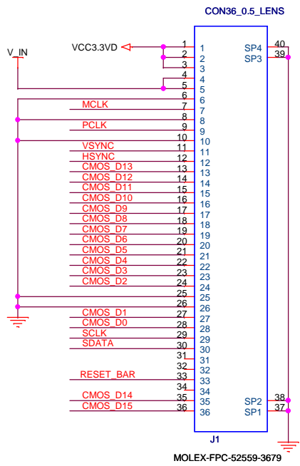
IP CAMERA COMPATIBLE CAMERA BOARD
